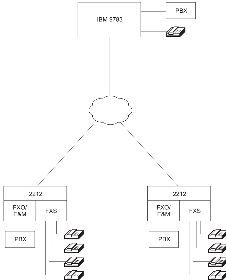
Figure 53. IBM 9783 to 2212 Voice Interfaces Communication
