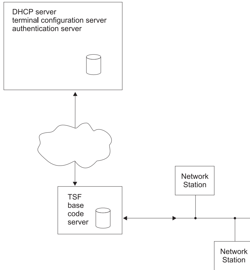
Figure 51. Remote Network Station with a Thin Server
