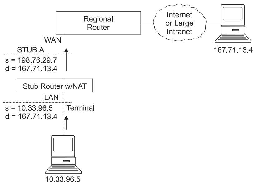
Figure 45. Network Running NAT
