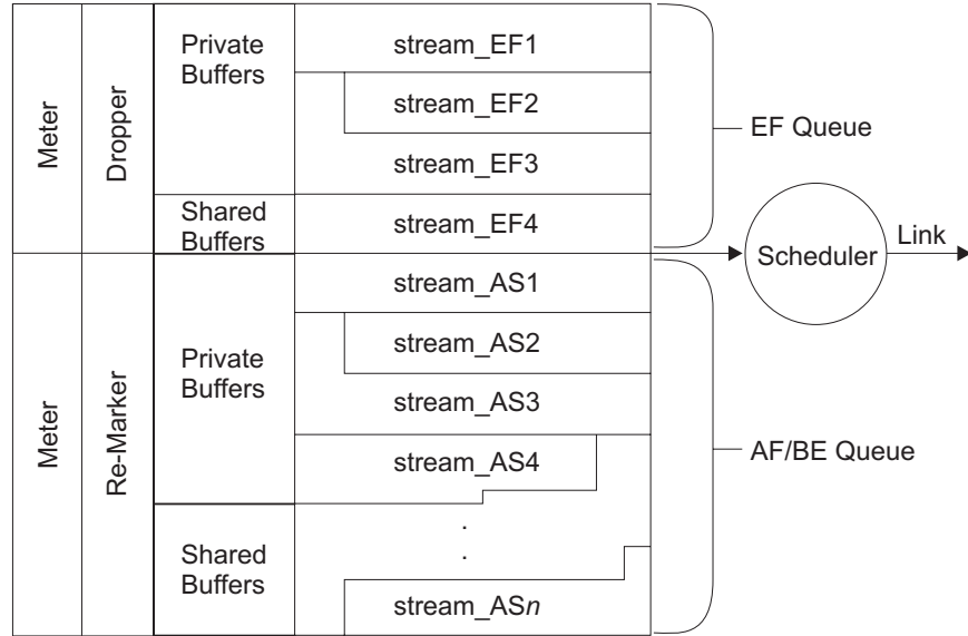
Figure 40. Relationship of Policers, Buffers, Queues, and Scheduler
