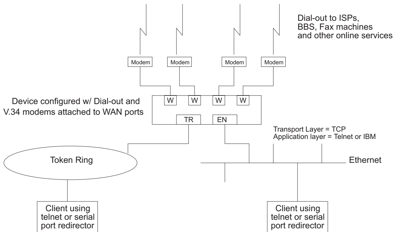
Figure 47. An Example of a DIALs Server Supporting Dial-Out
